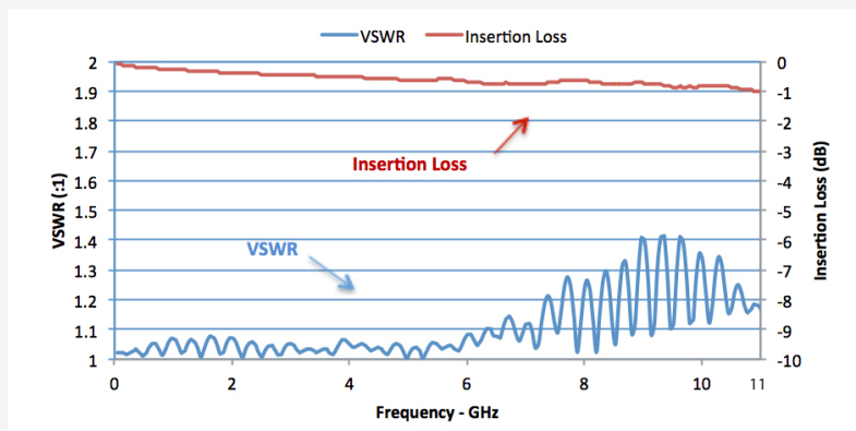
Typical performance data for 12" cable @+25°
